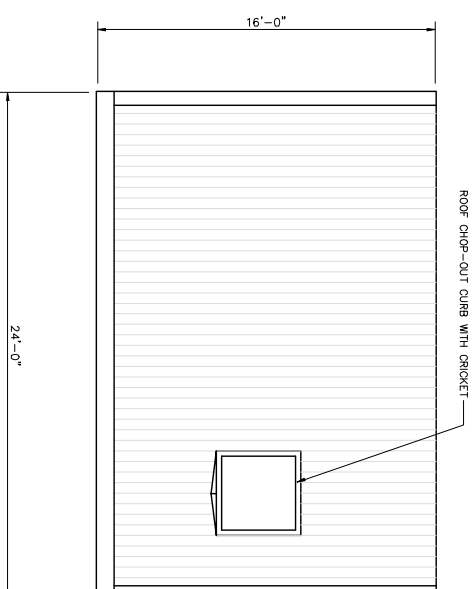
ROOF PLAN
