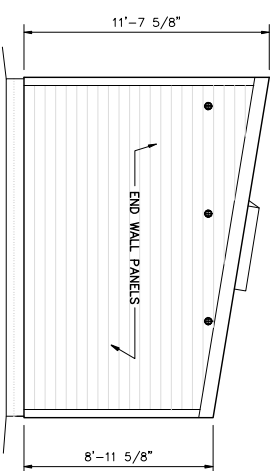
EAST END ELEVATION
