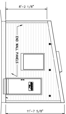
WEST END ELEVATION
