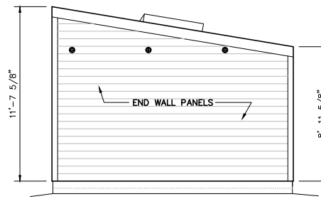
EAST END ELEVATION
