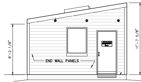
WEST END ELEVATION
